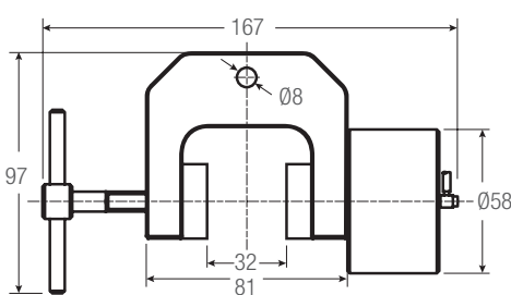
PNEUM-240KA-30-1
