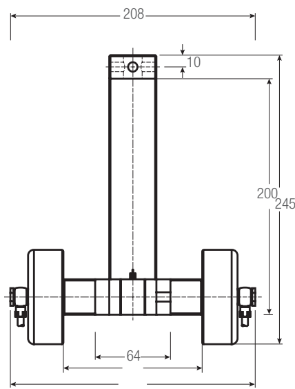
PNEUM-56GH2KA-1
