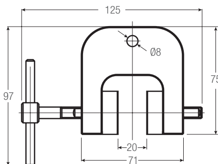
VISE-240KA-20-1
