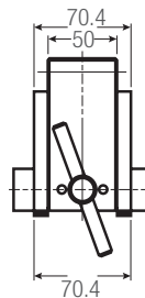
WISE-240G-S100
