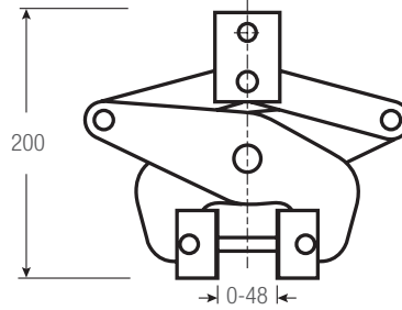
SCISSOR-11-50S-1
