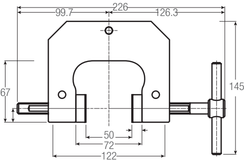
WISE-240G-S50
