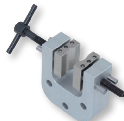
VISE-240KA-20-1
